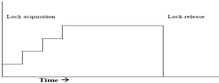
Strict Two Phase Locking
