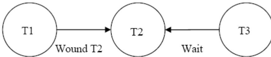
Wound-wait Scheme of Deadlock prevention
